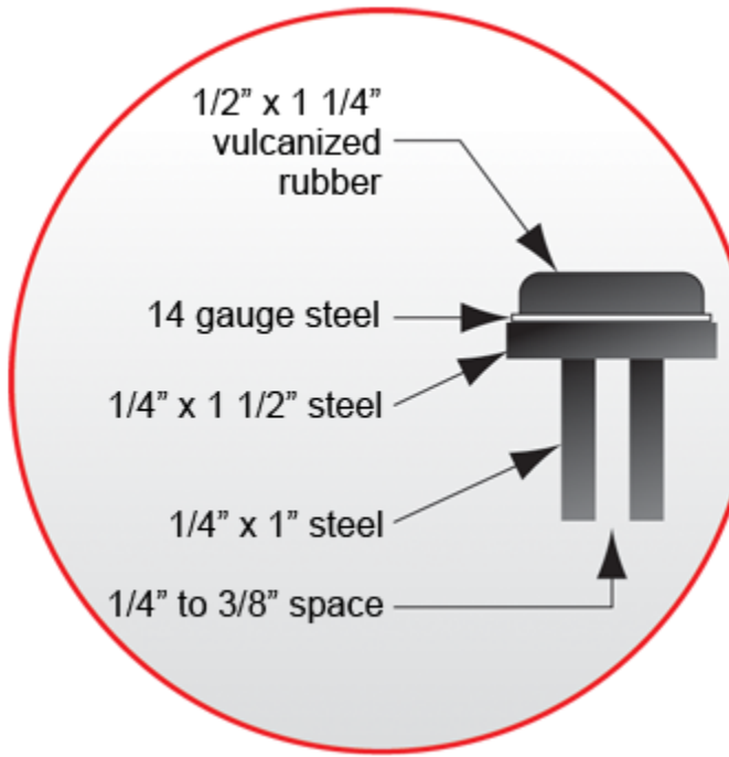
Replaceable Lagging Strip crosssection
